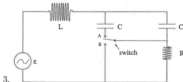
Figure 1: An AC circuit.
